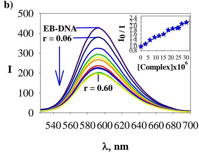
Şekil 4.18. Komplekslerin EB+CT-DNA ile etkileşimine ait floresans spektrumları (a) \{[\text{Cu}(\text{phen})(\text{gln})(\text{H}_2\text{O})]\text{NO}_3 \cdot \text{H}_2\text{O}\}_n (b) \{[\text{Cu}(\text{dmphen})(\text{gln})(\text{H}_2\text{O})]\text{ClO}_4\}_n
