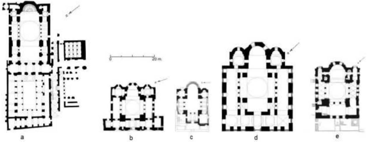
Plan 6: Aya İrinli Kilisesi (a), Koimesis Kilisesi (b), Klemens Kilisesi (c), Selanik Aya Sofya Kilisesi (d), Theodosios Kilisesi (Gül Camii) (e).
