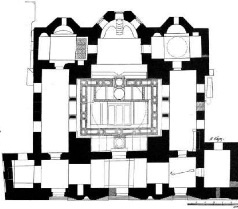
Plan 1: Koimesis Kilisesi Planı, (Schmit 1927 Tafel IV).
