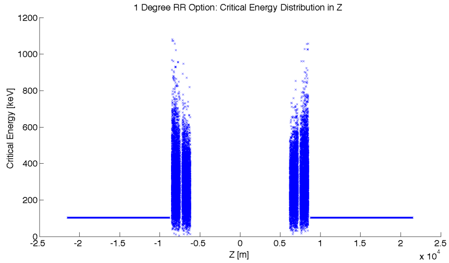
Figure 6.46: High Acceptance: Critical Energy Distribution in Z
