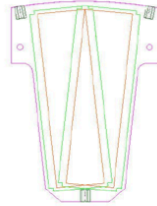
Figure 12.27: Proposed mechanics layout for the CMS tracker wheel upgrade.
