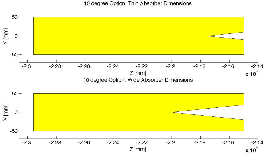
Figure 6.42: High Luminosity: Absorber Dimensions
