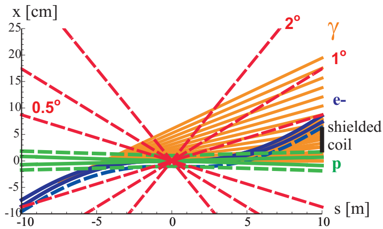
Figure 7.2: Linac-ring interaction-region layout. Shown are the beam envelopes of 10\sigma (electrons) [solid blue] or 11\sigma (protons) [solid green], the same envelopes with an additional constant margin of 10 mm [dashed], the synchrotron-radiation fan [orange], the approximate location of the magnet coil between incoming protons and outgoing electron beam [black], and a “1 degree” line.
