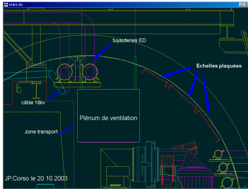
Figure 6.64: Air-duct in LSS7 indicated by the box labelled 'Plénum de ventilation' [683].
