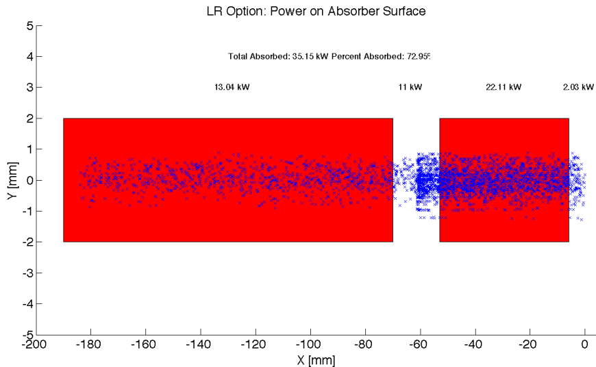
Figure 7.23: LR: Photon distribution on the Absorber Surface.
