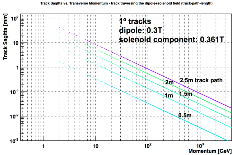
Figure 12.22: Track Sagitta vs. momentum of 1^\circ -tracks in a superposed dipole (0.3T) and solenoidal field component (0.361T).
