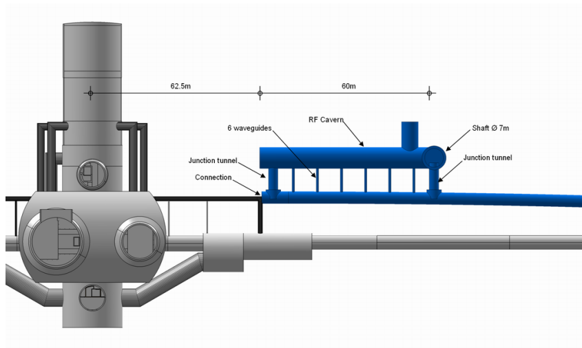
Figure 8.16: RF tunnel Layouts at CMS and ATLAS bypasses. Note only the right hand side at ATLAS shown.
