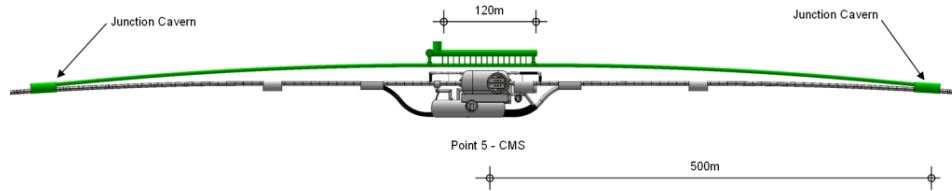
Figure 9.5: Ring-Ring Bypass around CMS Point 5.
