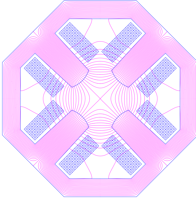
Figure 8.14: Quadrupoles for the 10 GeV linacs of the LR option (scale 1:5).
