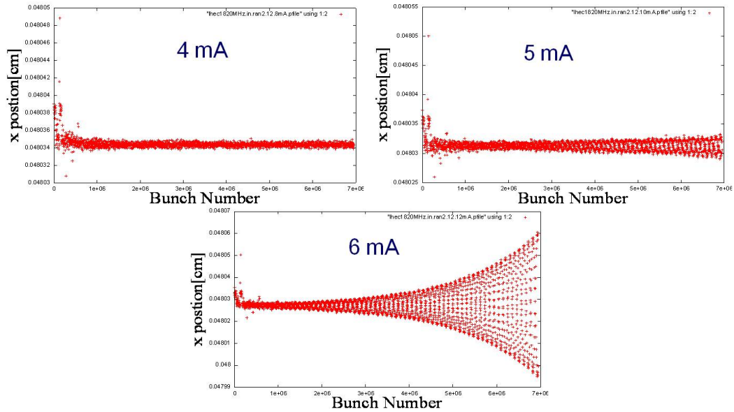
Figure 7.40: Large scale TDBBU simulation results for various beam currents: 4 (top left), 5 (top right) and 6 mA.
