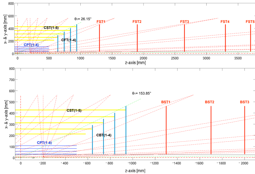
Figure 12.20: LicToy2.0 tracker design of the central/forward FST(top) and central/backward direction BST(bottom).
