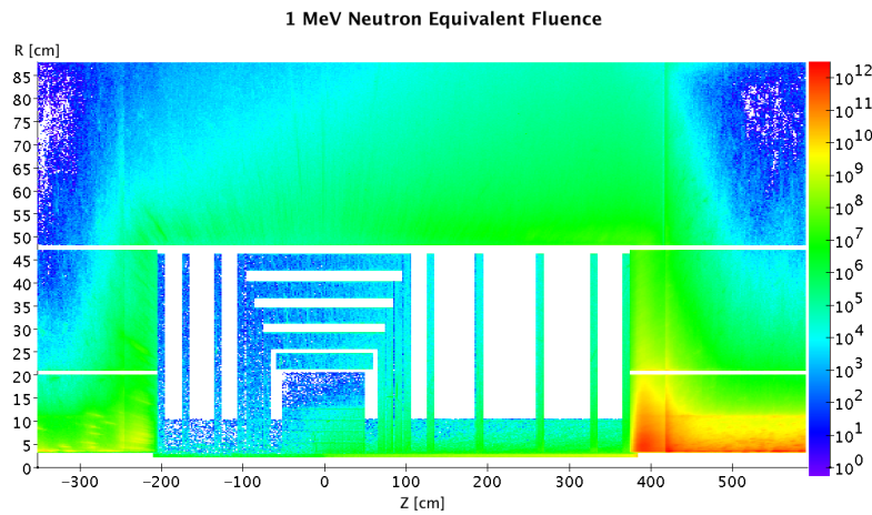
Figure 12.60: 1 MeV Neutron Equivalent Fluence [ cm^{-2}/year ].
