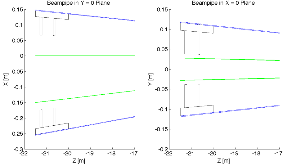
Figure 6.49: High Acceptance: Beam pipe Cross Sections
