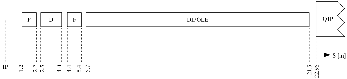
Figure 6.25: Layout of machine elements in the HL IR. Note that the left side of the IR is symmetric.
