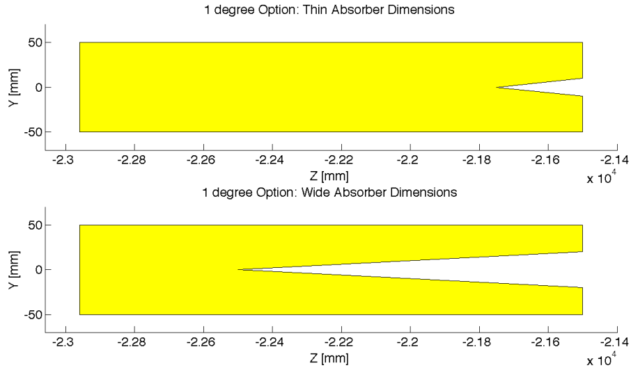
Figure 6.48: High Acceptance: Absorber Dimensions
