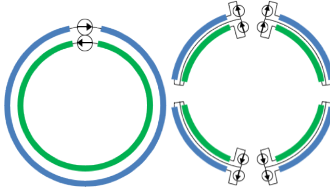
Figure 8.24: Different possibilities to power the MQ magnets.
