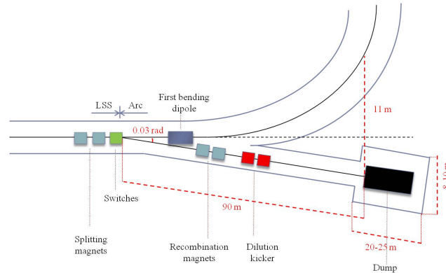
Figure 8.46: Scheme of the transfer line from end of long straight section of the linac and beam dump.
