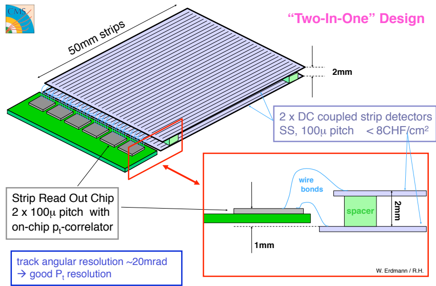
Figure 12.23: Layout of the 2_in_1 strip sensor design used as p_t -trigger setup for the CMS experiment.
