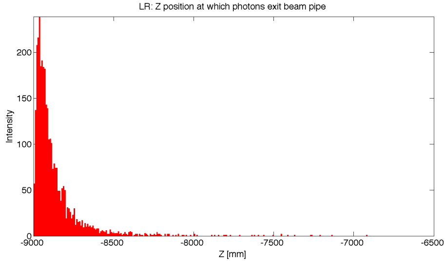
Figure 7.27: LR: Backscattered Photons Exiting the Beam Pipe.
