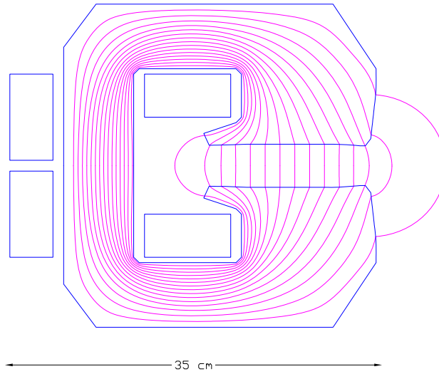
Figure 8.9: Bending magnets for the RR option (scale 1:5).
