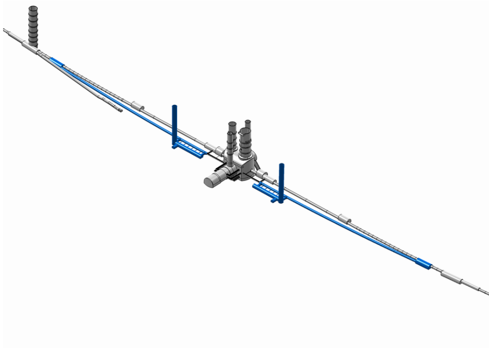
Figure 9.6: Ring-Ring Bypass around ATLAS Point 1.
