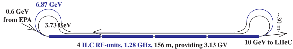
Figure 6.67: Recirculator using 4 ILC modules.
