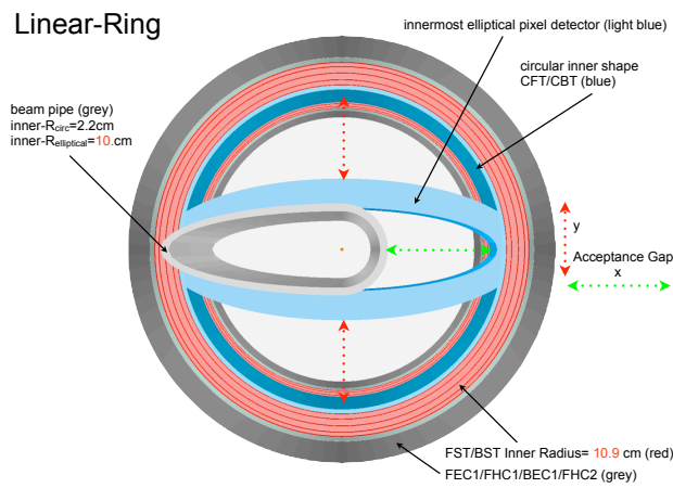
Figure 12.7: Linac-Ring beam pipe design and acceptance gaps due to deviations in shape of the forward/backward tracking detectors FST/BST (circular) and the innermost central pixel detector layer (elliptical) from the beam pipe shape.
