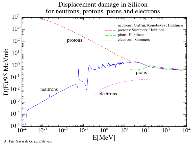
Figure 12.59: Displacement Damage for various particles in Silicon
