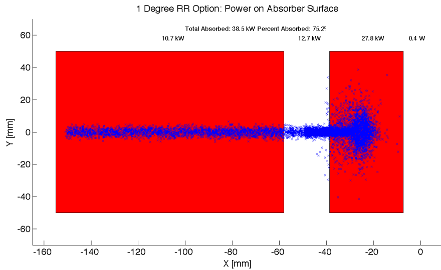
Figure 6.47: High Acceptance: Photon distribution on Absorber Surface
