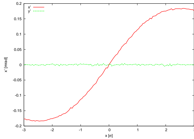
Figure 7.7: Simulated electron horizontal centre-of-mass deflection angle as a function of the horizontal beam-beam offset.
