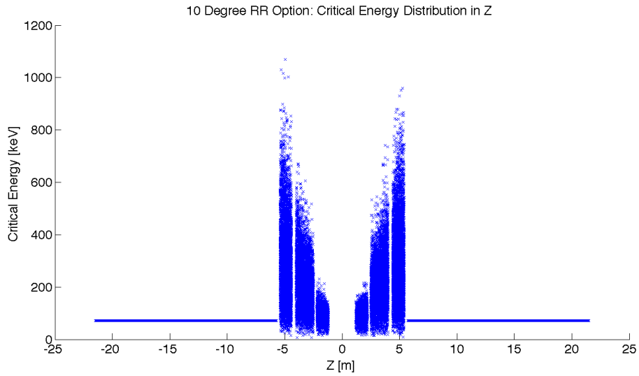
Figure 6.40: High Luminosity: Critical Energy Distribution in Z
