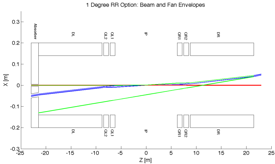
Figure 6.45: High Acceptance: Beam Envelopes in Z
