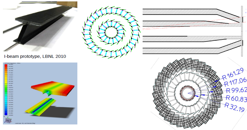
Figure 12.25: Proposed mechanics and sensor layout for the ATLAS pixel upgrade.
