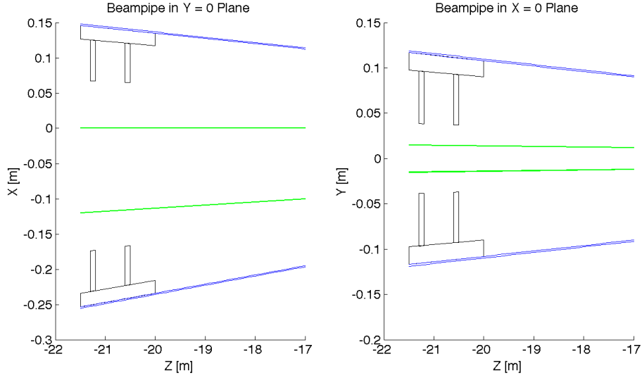
Figure 6.43: High Luminosity: Beam pipe Cross Sections
