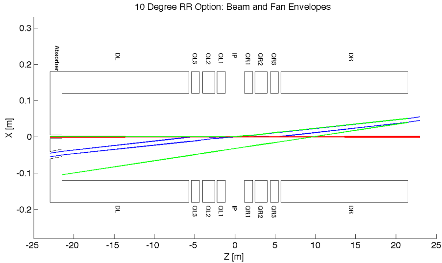
Figure 6.39: High Luminosity: Beam Envelopes in Z
