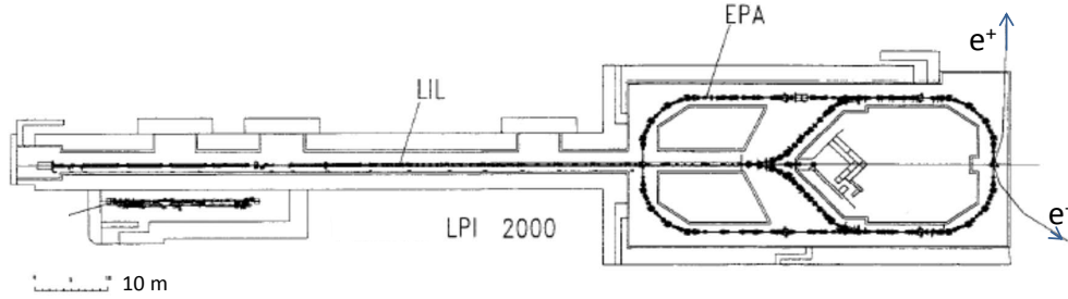
Figure 6.65: Layout of the LPI in 2000.
