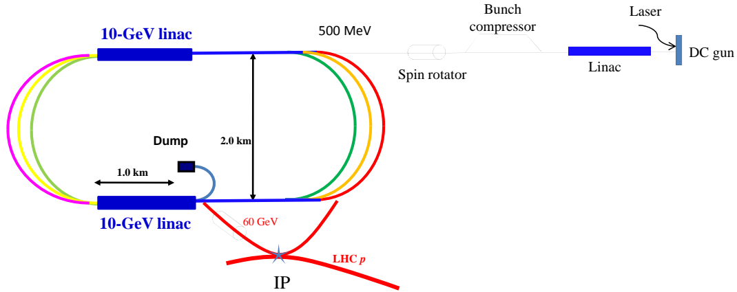
Figure 7.45: Layout of the injector (not to scale).
