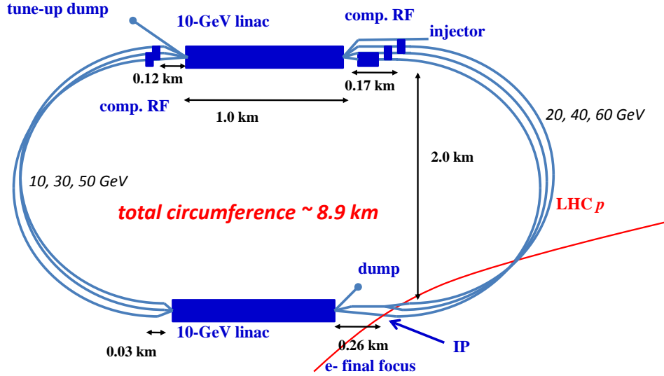
Figure 7.5: LHeC ERL layout including dimensions.
