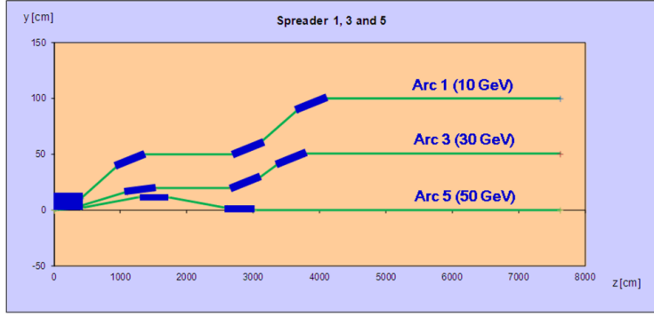
Figure 7.32: Vertical spreader architecture based on one common “splitter” magnet.
