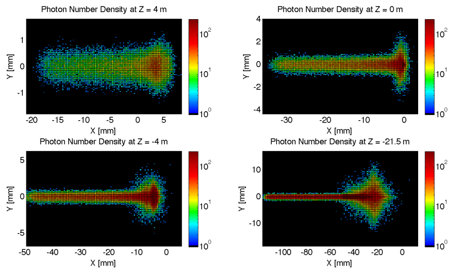
Figure 6.38: High Luminosity: Number Density Growth in Z
