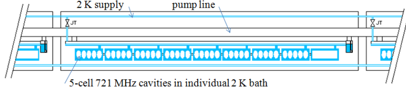
Figure 8.36: Schematic proposal of the 14 m long cryomodules with eight 5-cell 721 MHz cavities operating at 2 K. Supply pipes and the 30 mbar pump line are within cryostat envelope. For the case with inclination right part is lower (only 2 K circuits are shown).
