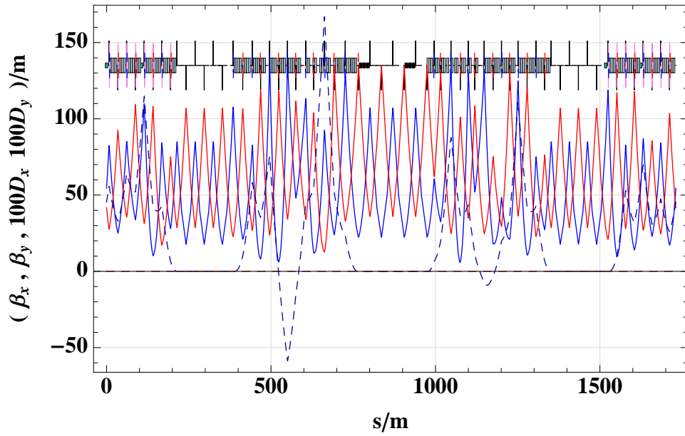
Figure 6.14: Bypass optics Point 1.
