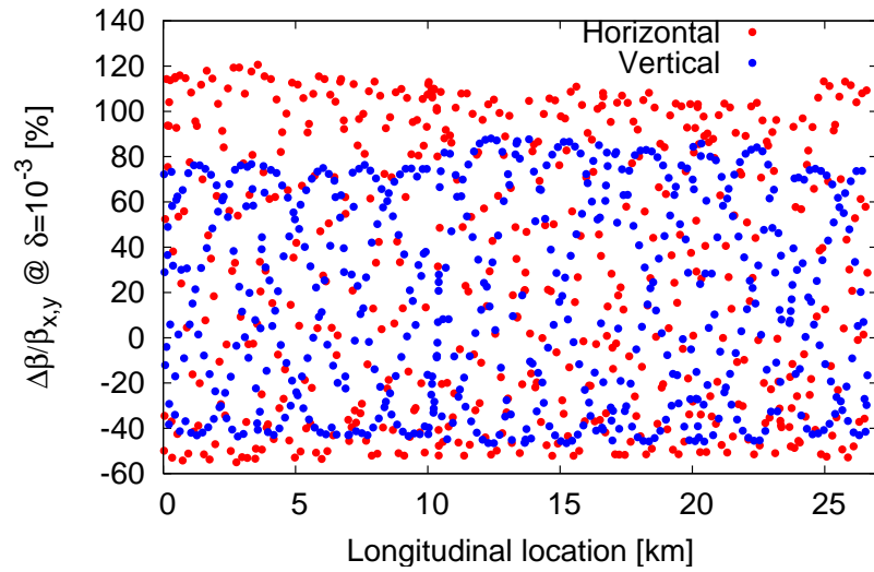
Figure 7.16: Chromatic beta-beating at dp/p=0.001 .
