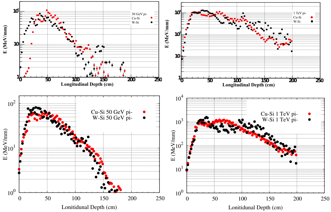
Figure 12.49: Comparison of FEC_{(W-Si)} \& FHC_{(Cu-Si)} (red) and FEC_{(W-Si)} \& FHC_{(W-Si)} (black) stack systems in terms of average energy depositions as a function of stack depth for pions of energy 50\text{ GeV} (left) and the same comparison for pions with energy 1\text{ TeV} (right) ( GEANT4 (top) and FLUKA (bottom)).
