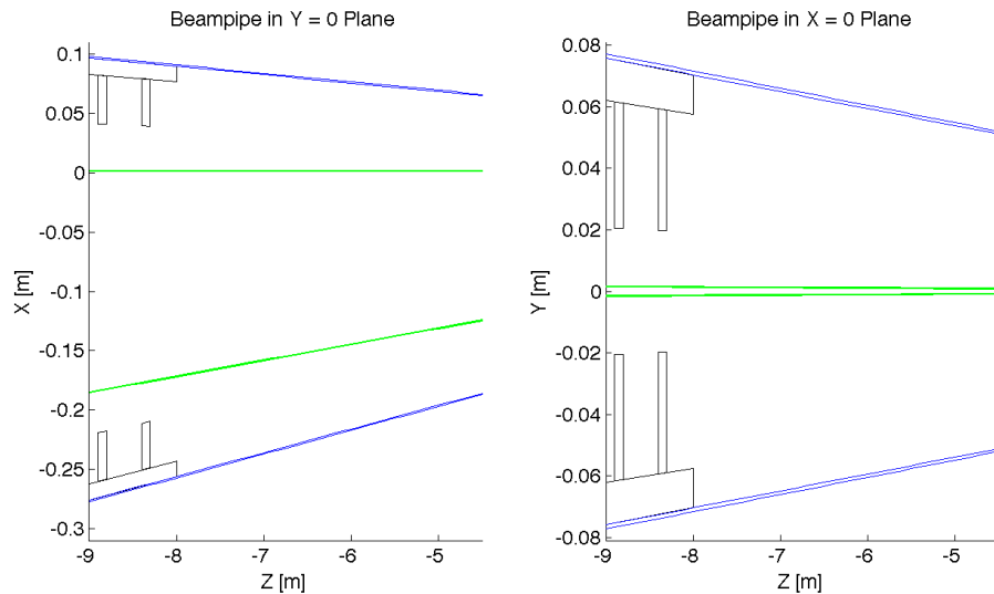
Figure 7.28: LR: Beam pipe Cross Sections.
