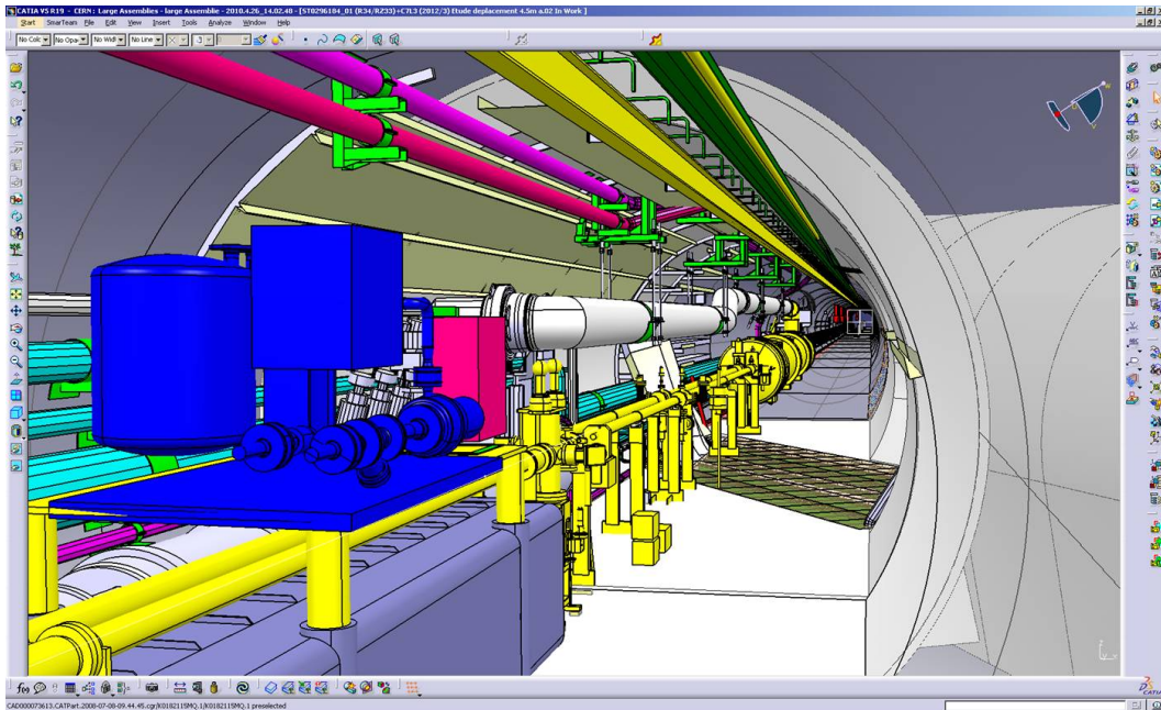
Figure 6.61: The cryogenic connection in Point 3
