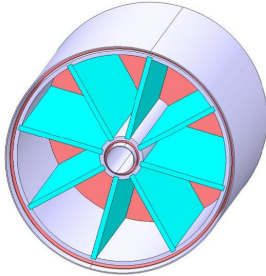
Figure 12.56: CAD drawing for a 2T air core toroid with 20 cm bore and a size about 1 \text{ m}^3
