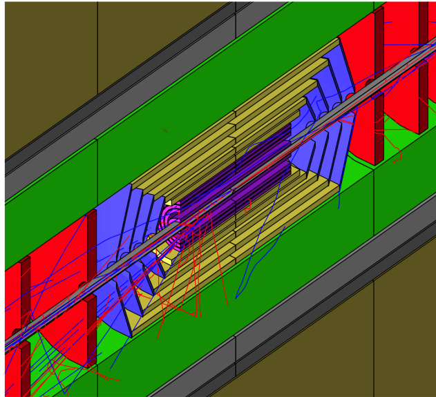
Figure 12.63: G4 Event
