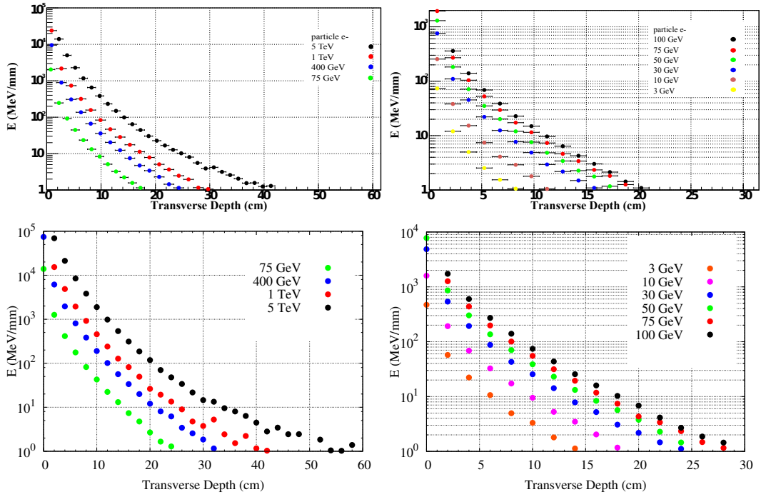
Figure 12.46: Comparison of transverse shower profiles for electrons with energies 75 GeV-5 TeV on FEC_{(W-Si)} (left) and 3 GeV-100 GeV on BEC_{(Pb-Si)} (right) ( GEANT4 (top) and FLUKA (bottom)).
