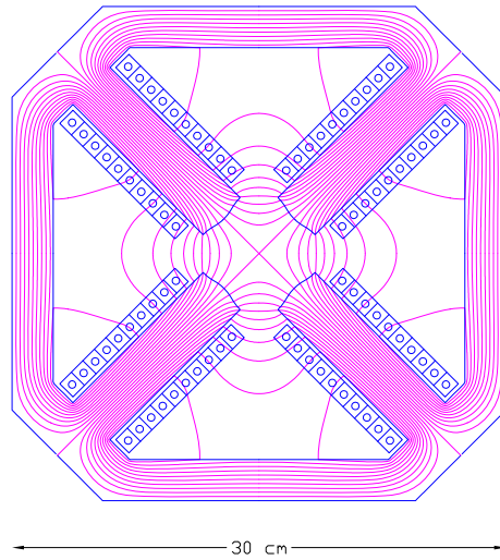
Figure 8.10: Arc quadrupoles for the RR option (scale 1:5).
