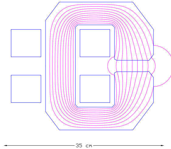
Figure 8.12: Bending magnets for the LR recirculator (scale 1:5).
