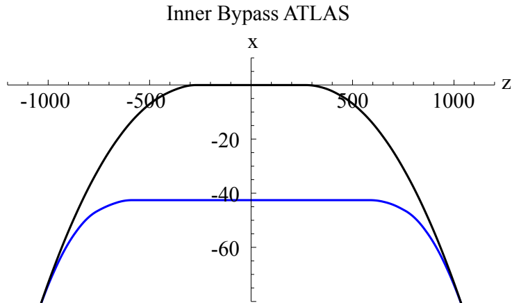
Figure 6.9: Example of an inner Bypass around Point 1. The Bypass is shown in blue, The LHC proton ring in black.
