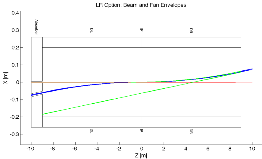
Figure 7.22: LR: Beam Envelopes in Z direction.
