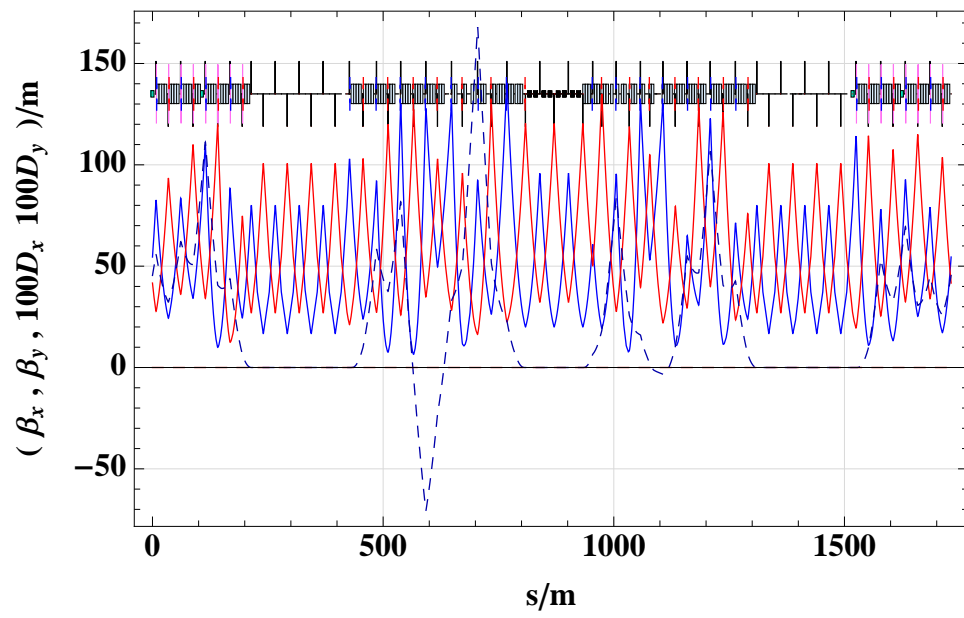
Figure 6.15: Bypass Optics Point 5.
