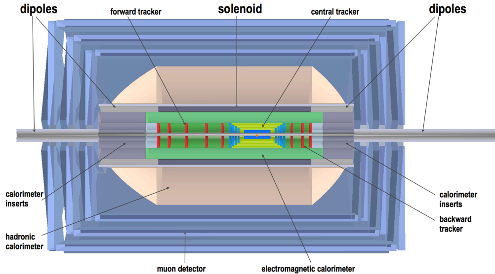
Figure 12.12: Configuration of the solenoid and electron beam bending dipoles in the baseline Linac-Ring detector. Longitudinal r - z section showing the position of the solenoid and the two dipoles, each split in two sections, a superconducting inner section incorporated with the solenoid in one cryostat and a normal conducting iron based outer section magnet with smaller bore.
