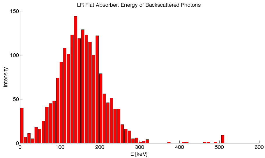
Figure 7.26: LR: Backscattered Energy Distribution.
