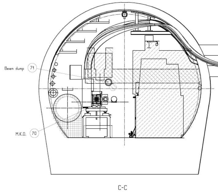
Figure 6.56: Dump kicker [682]
