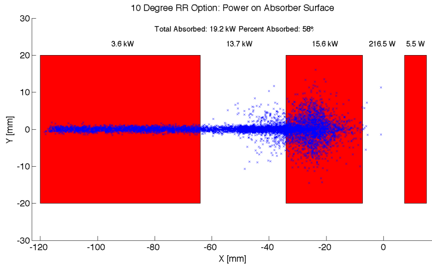
Figure 6.41: High Luminosity: Photon distribution on Absorber Surface
